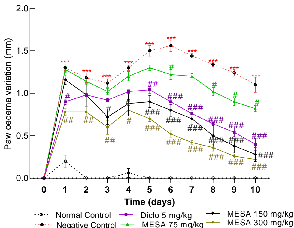
Figure 1: Effect of MESA on the evolution of edema during formaldehyde-induced inflammation Values are presented as means \pm SEM, (n = 5). Significant differences compared to control groups are indicated as follows: *** P < 0.001 compared to the normal control; # P < 0.05 , ## P < 0.01 , and ### P < 0.001 compared to the negative control. MESA: Methanolic Extract of S. aethiopicus ; Dilco: Diclofenac.
