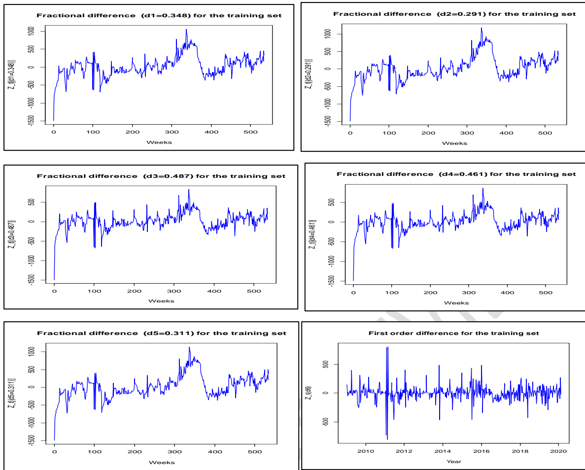
Figure 3. Fractional difference series and first order difference series
