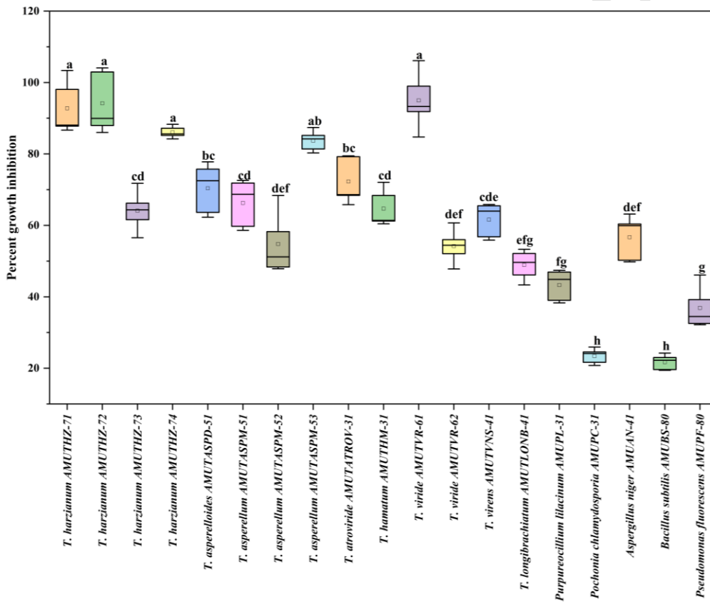
Figure 1. In-vitro , the effect of biocontrol fungi and bacteria on the percent growth inhibition of Macrophomina phaseolina AMUMP-2. Different alphabets are indicated significantly different at P \leq 0.05 according to Tukey test. Error bars show standard deviation
