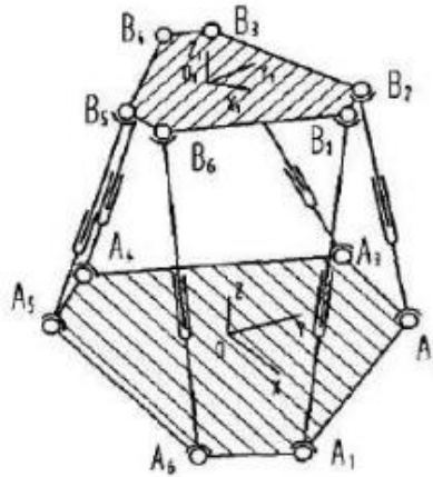
Figure 1 Structure diagram of the parallel robot
