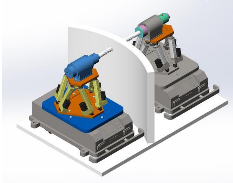
Figure 2 Mobile multi-robot processing platform
