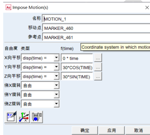
Figure 4 Setting the tool function
