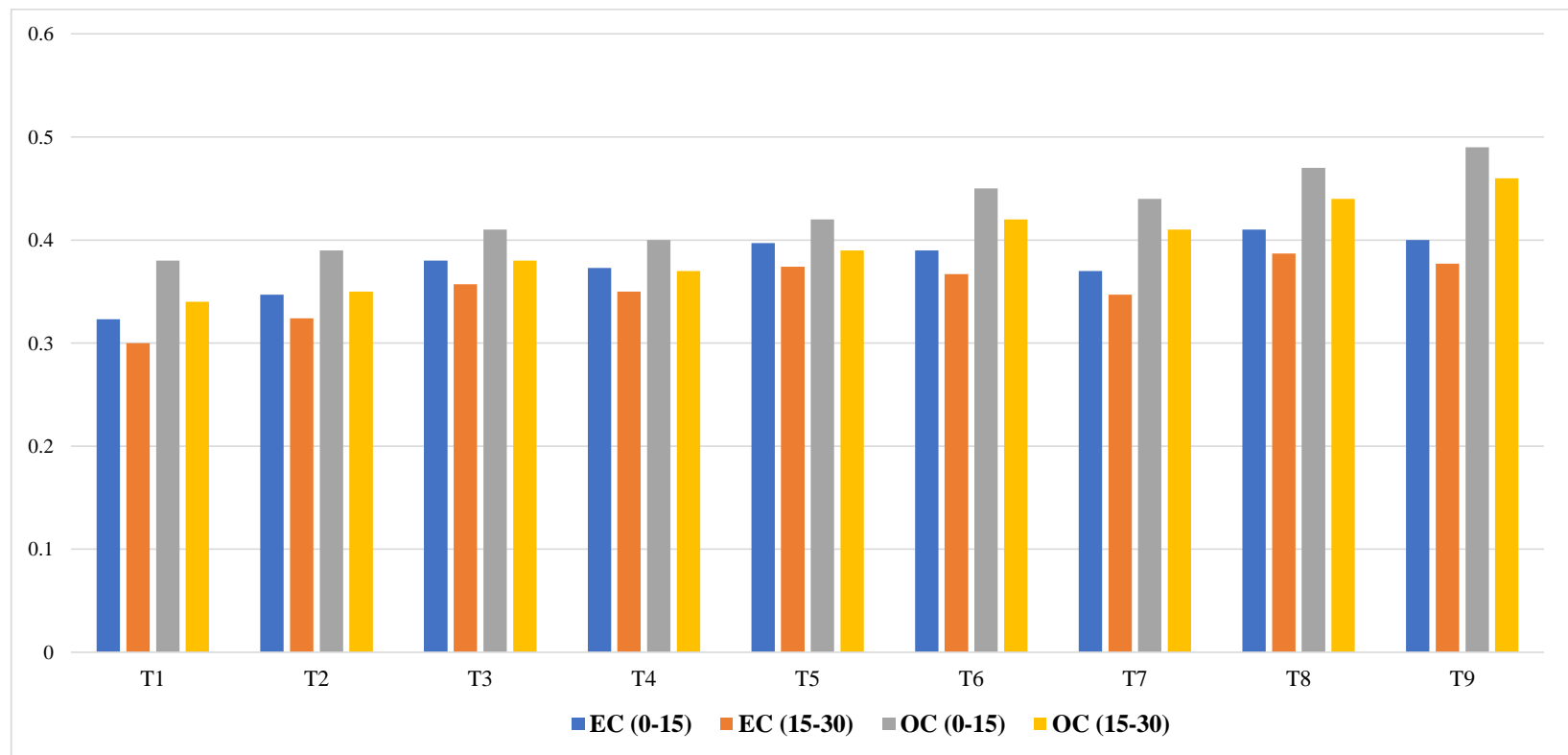
Fig. 2. Effect of Different Levels of NPK and Rhizobium on Electrical conductivity and Organic carbon.
