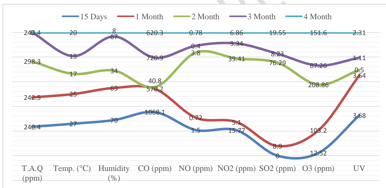
Fig. 2: Variable gas concentrations at the under-road traffic site
