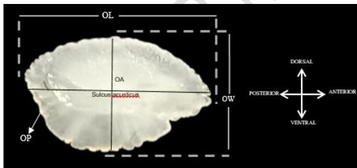
Fig 1. Otolith morphometric measurement axis. Otolith length (OL), otolith width (OW), otolith perimeter (OP), otolith area (OA).
