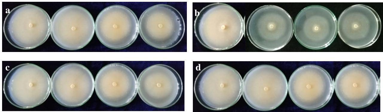
Figure 1: Compatibility of a) Trifloxystrobin b) Azoxystrobin c) Kresoxym methyl d) Pencycuron with P. indica at 100, 250 and 350 ppm concentrations. P. indica is grown on PDA amended with respective fungicides and mycelial growth was recorded at various time intervals
