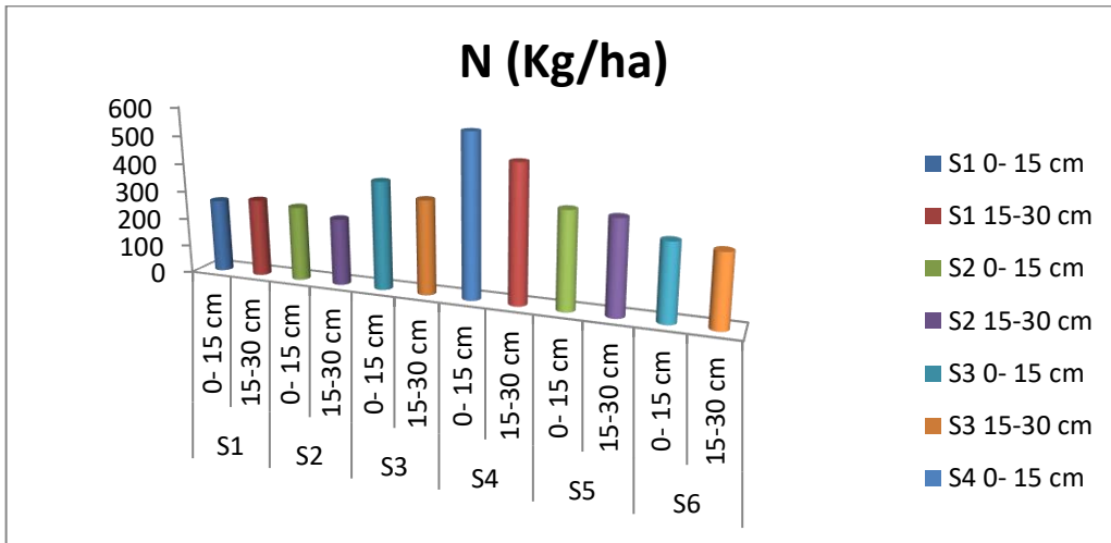
Fig. 4 soil nitrogen in different cropping system
