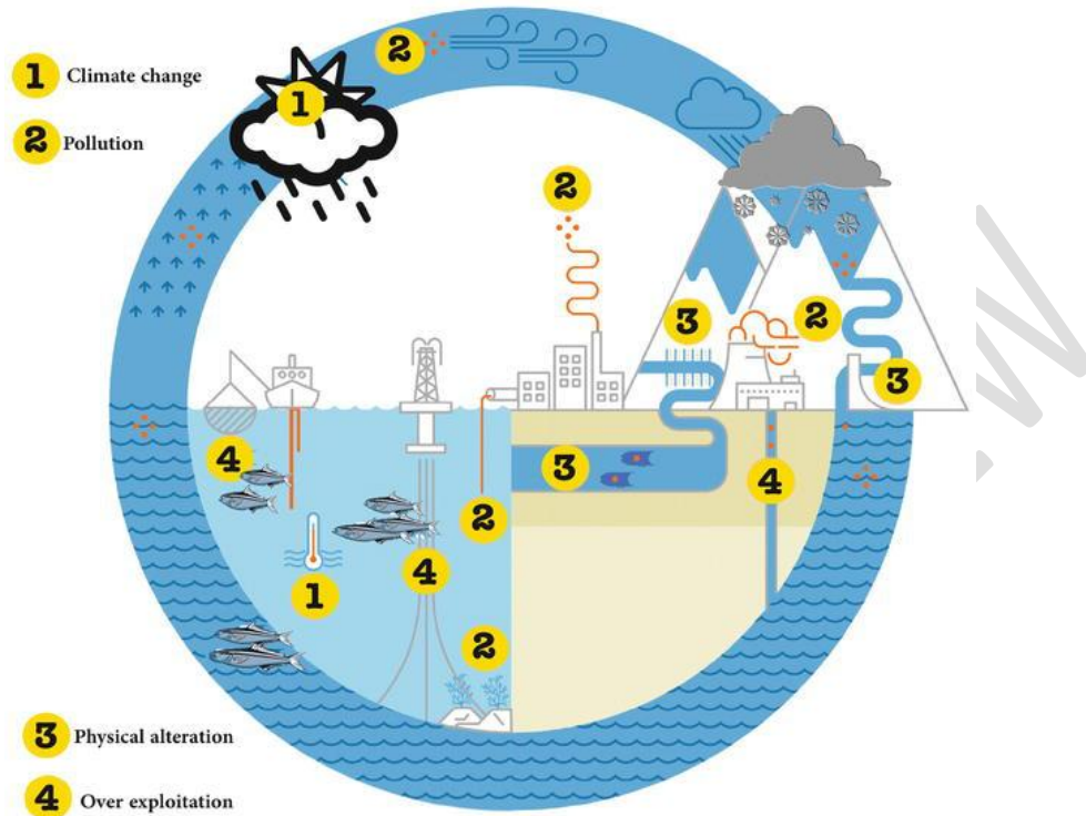
Fig: Water cycle and pressure factors and areas of application of AI [Source:EEA Signals 2018]. Legend: 1) climatic change, 2) pollution, 3) physical alterations, 4) over exploitation.
