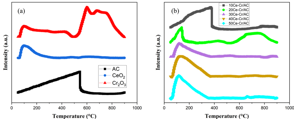
Fig. 7. NH 3 -TPD of the pure (a) and modified catalyst (b)
