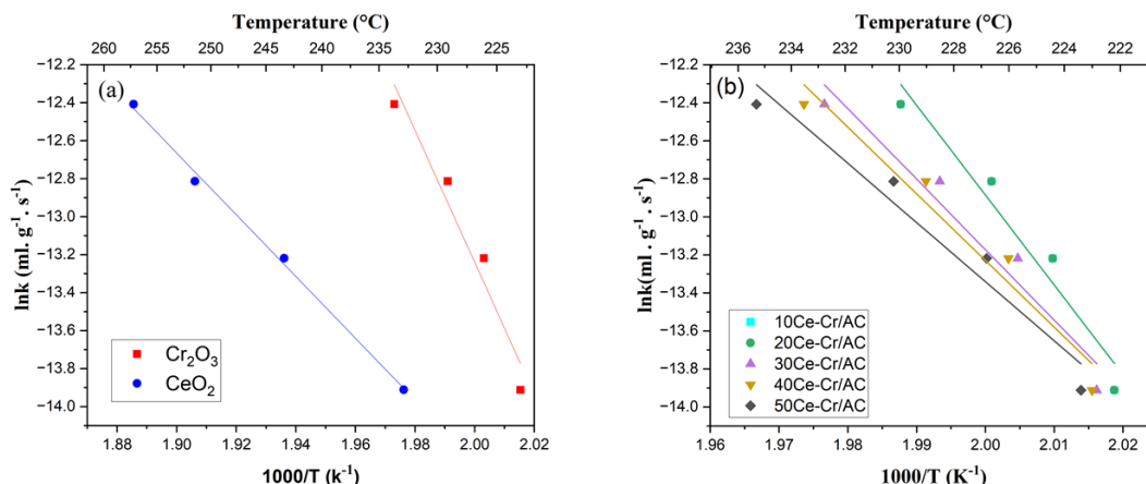
Fig. 9. Arrhenius plots of the pure (a) and modified catalyst (b)
