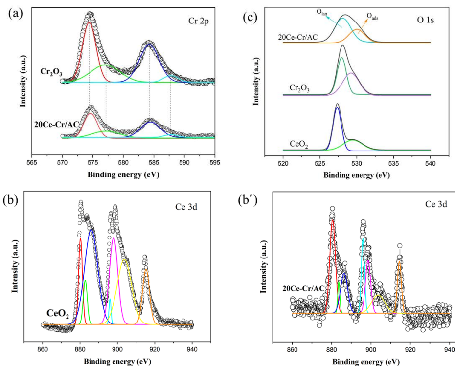
Fig. 5. The XPS spectra of m-Cr, p-Ce and 20Ce-Cr/AC catalysts. (a) Cr 2p; (b) Ce 3d and (c) O 1s
