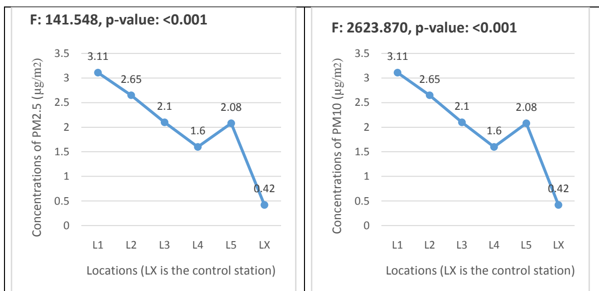
Figure 5: Line graph showing the levels SPM for PM 2.5 and PM 10
