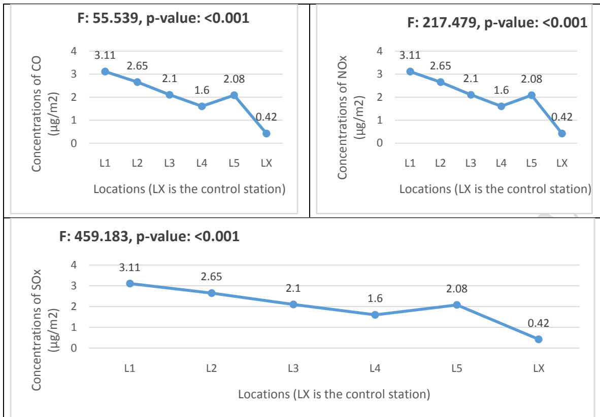
Figure 4: Line graph showing the difference in the CO, NO and SO levels in air samples from the sampled sites
