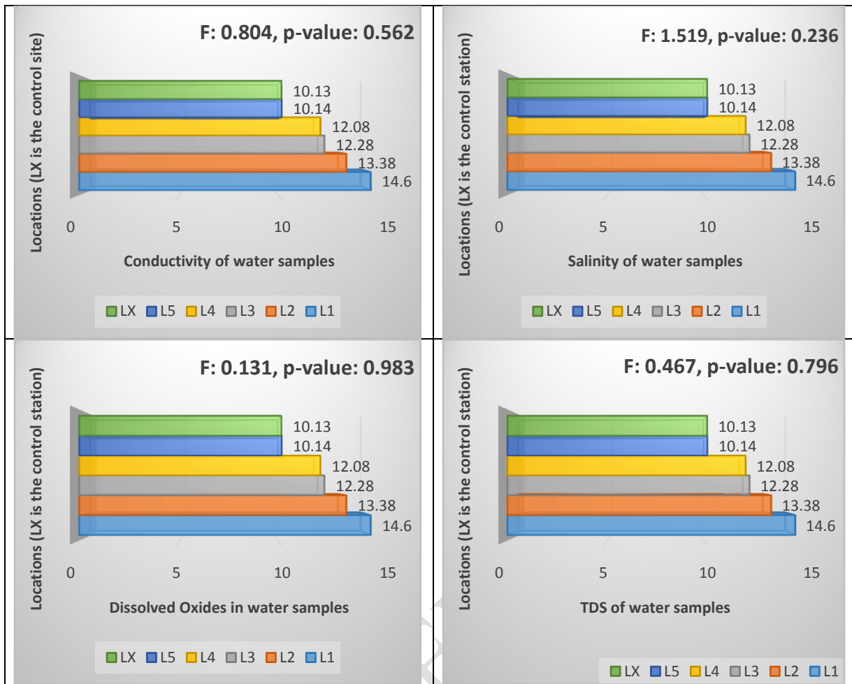
Figure 3: Bar chart showing the conductivity, salinity, dissolved oxides and total dissolved solids of the water samples
