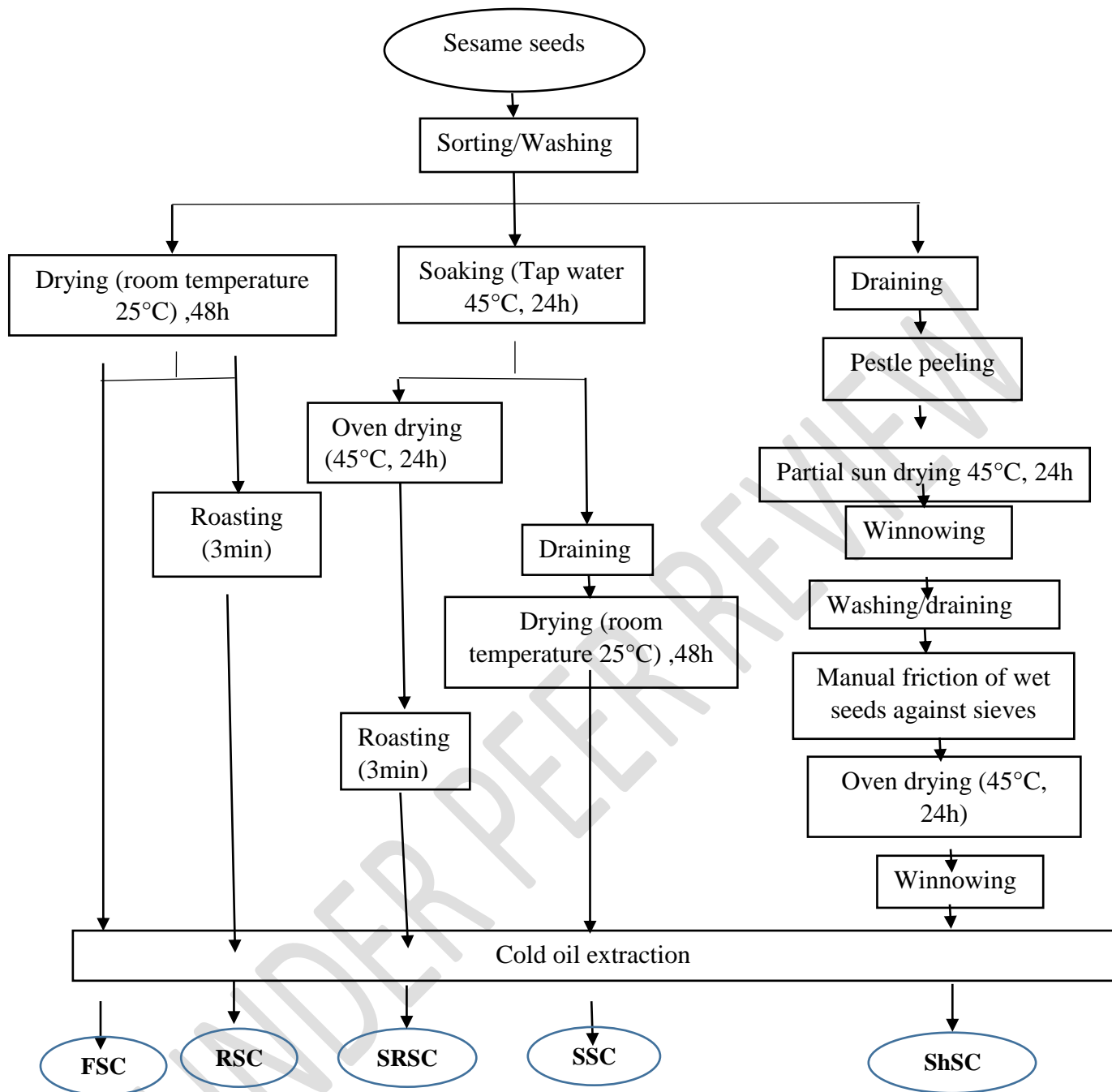
Figure 1: Sesame cake concentrate production diagram.
