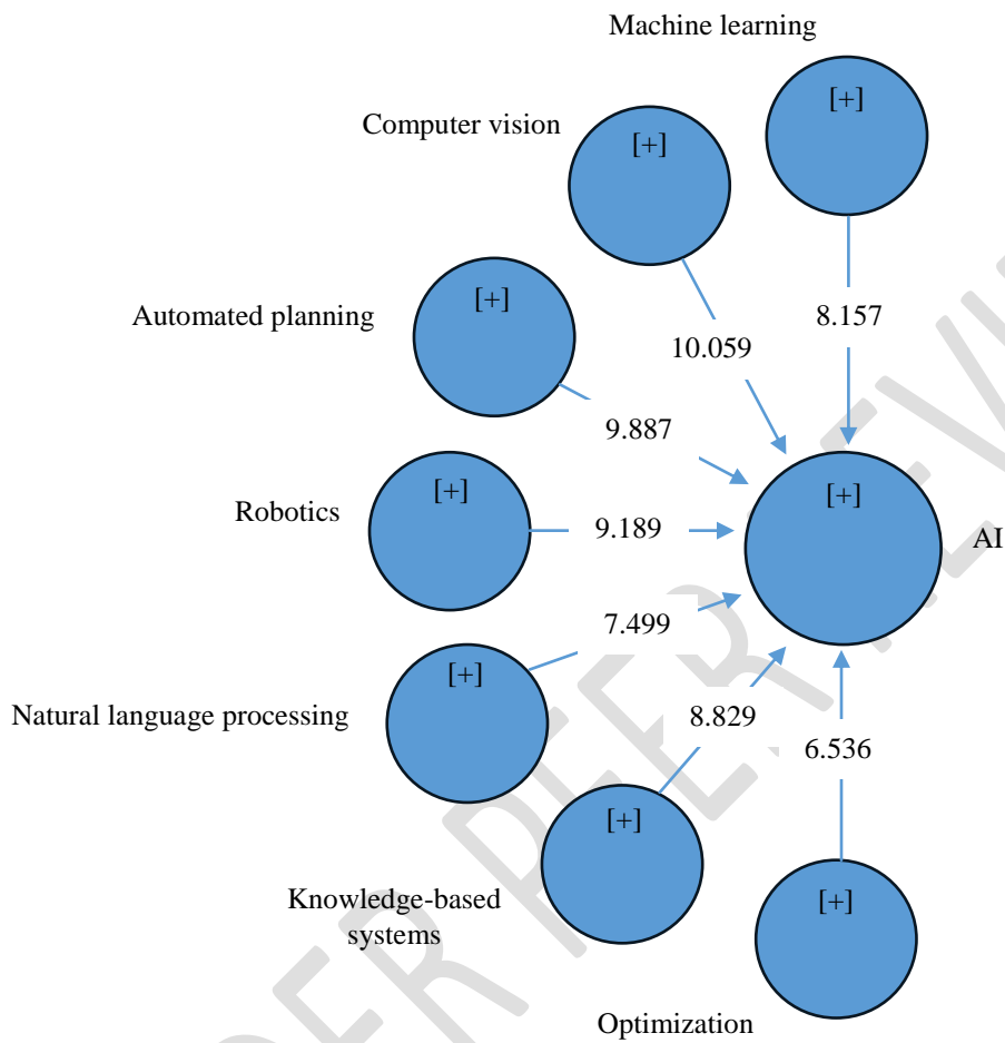
Chart 2- Measurement of the overall model in significance mode
