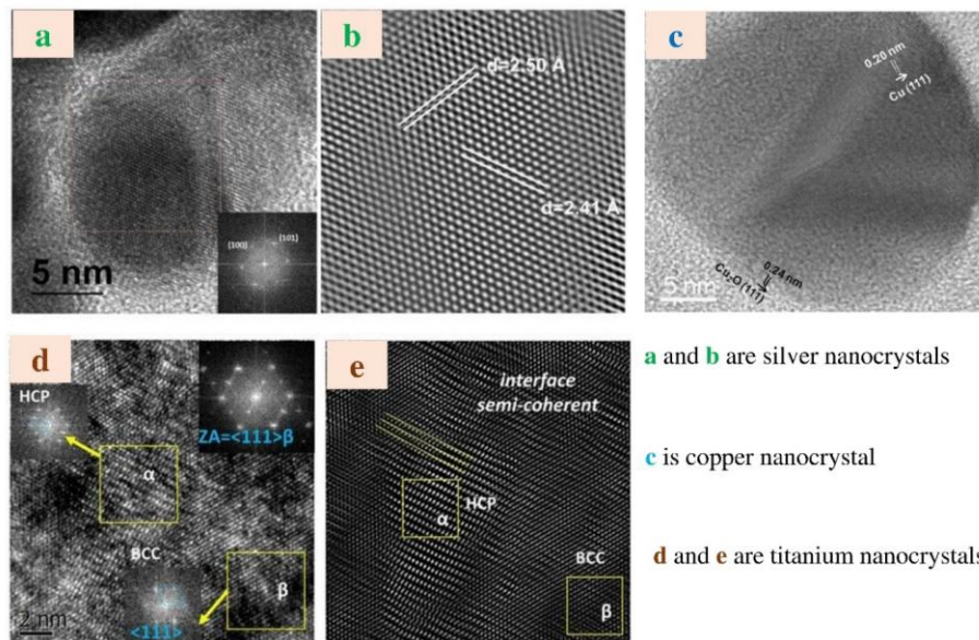
Fig. 7. HR-TEM of Ag [119], Cu [120] and Ti [121] nanocrystals
