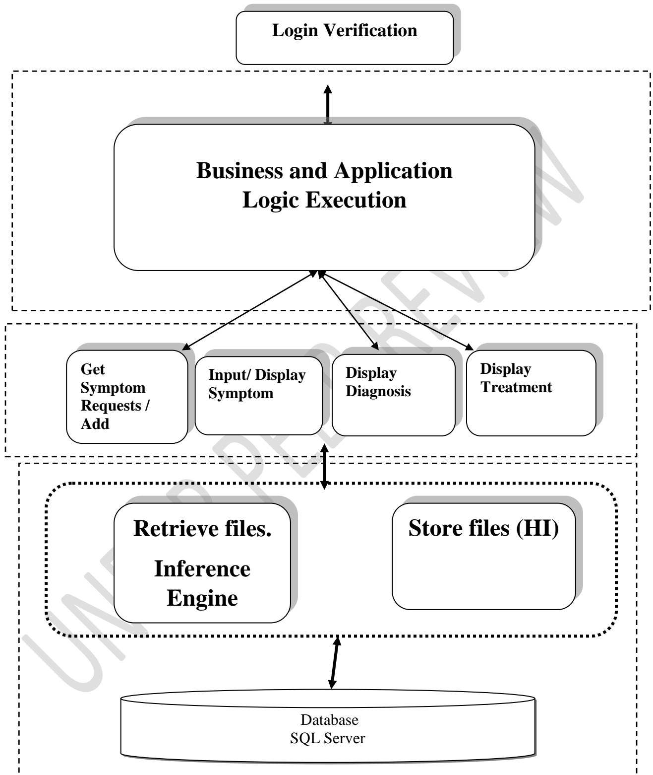
Fig 4. Login verification model
