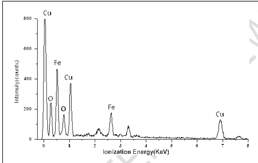
Fig. 2 EDX pattern of Cu doped FeO Nanoparticles
