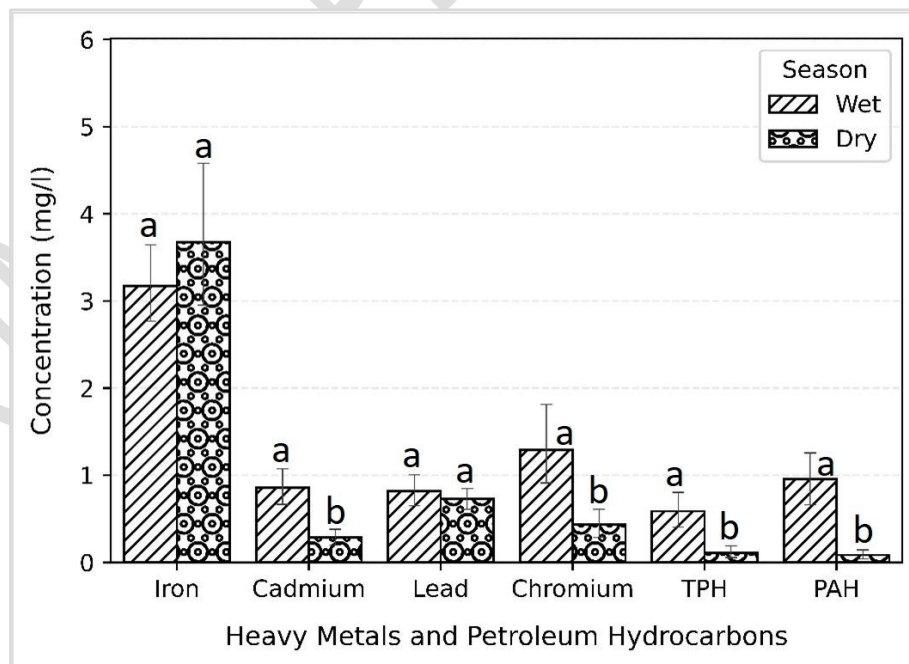
Figure 5: Concentration of heavy metals and petroleum hydrocarbons for the dry and wet season
