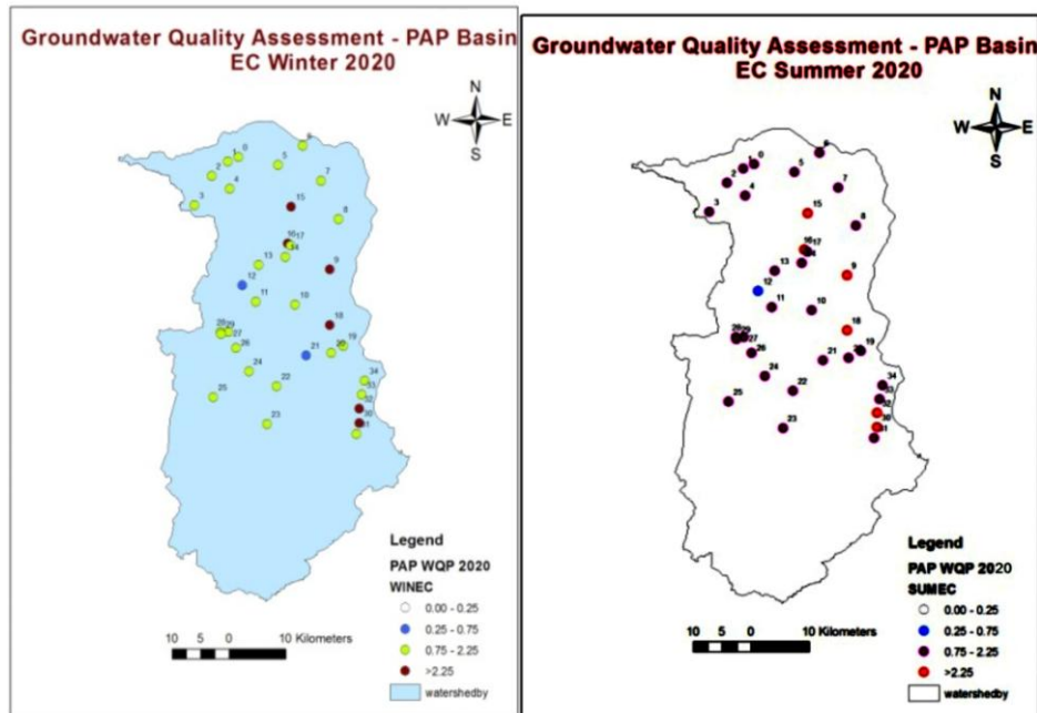
Fig 5. EC value in the groundwater samples of pap basin in various seasons of 2020
