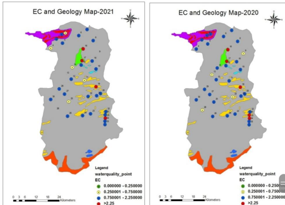
Fig. 7. EC in the ground water samples with geology (2020 and 2021)
