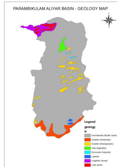
Fig.3 Geology map of PAP basin
