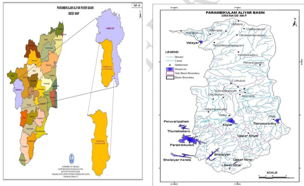
Fig. 1. Location and drainage map of the PAP basin (Source: PWD)
