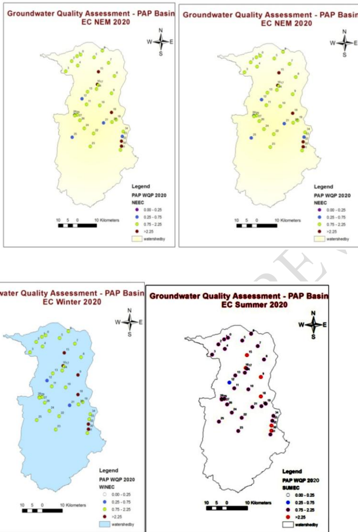
Fig 5. EC value in the groundwater samples of pap basin in various seasons of 2020
