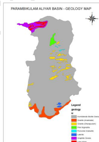
Fig.3 Geology map of PAP basin
