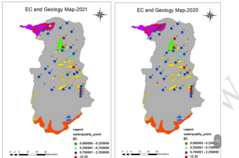
Fig. 7. EC in the ground water samples with geology (2020 and 2021)
