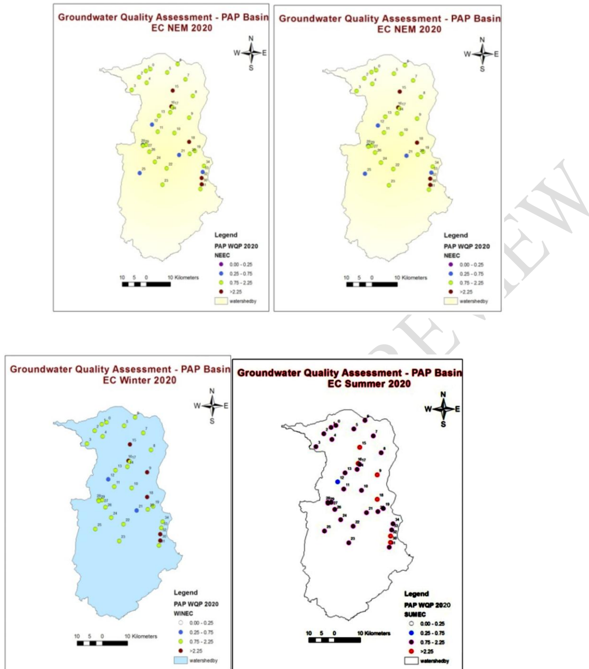
Fig 5. EC value in the groundwater samples of pap basin in various seasons of 2020
