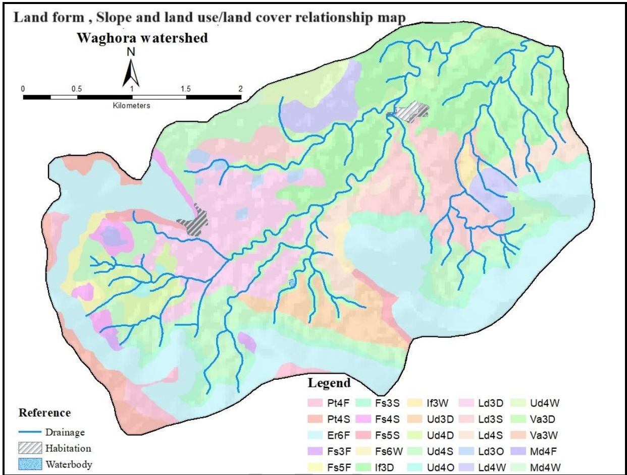
Fig. 5 Landform, Slope and Landuse/land cover relationship in Waghora watershed
