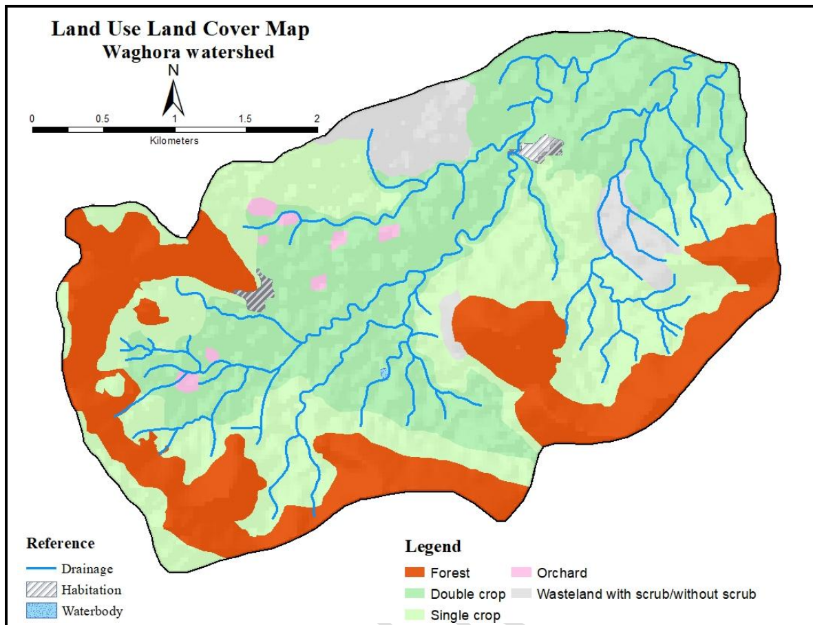
Fig.4 Land use/land cover map of Waghora watershed derived from Sentinel-2B (September 24, 2017 and January 27, 2018) data
