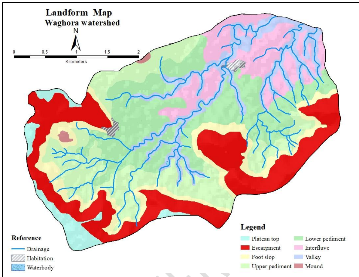
Fig. 3 landform of Waghora watershed derived from SRTM-DEM data
