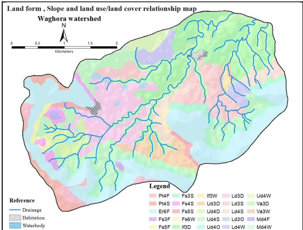
Fig. 4 Landform, Slope and Landuse/land cover relationship in Waghora watershed
