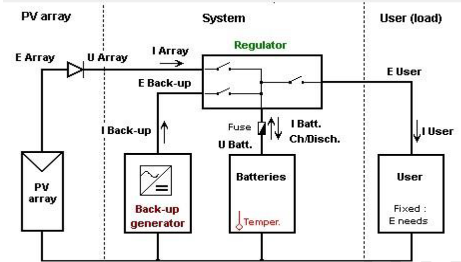
Fig 2:Schematic backup system layout in PVSyst software.
