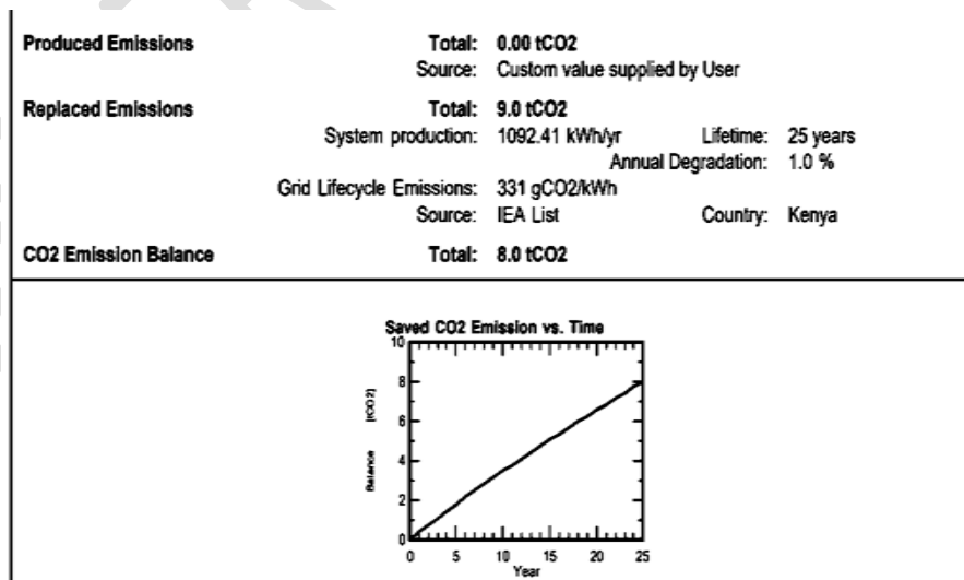
Fig 7: CO 2 balance
