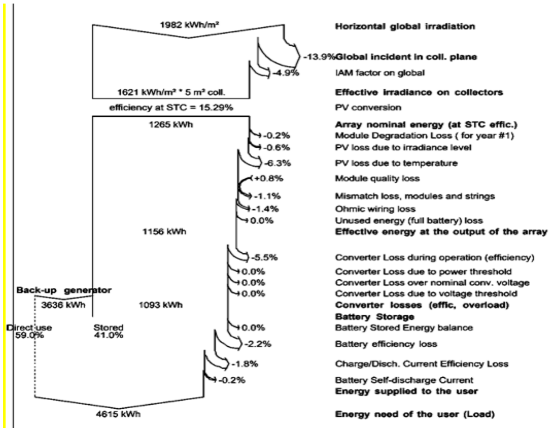
Fig 5. PVsyst Loss Diagram over the whole year
