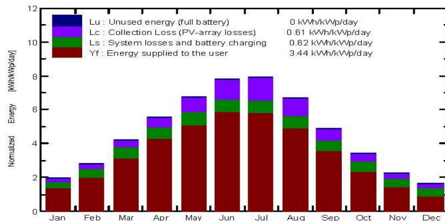
Fig 3. PVsyst monthly result report of normalized energy
