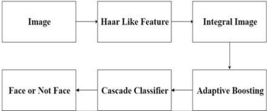
Fig. 4. The Cascade scheme classifier face detection process with Viola-Jones method.
