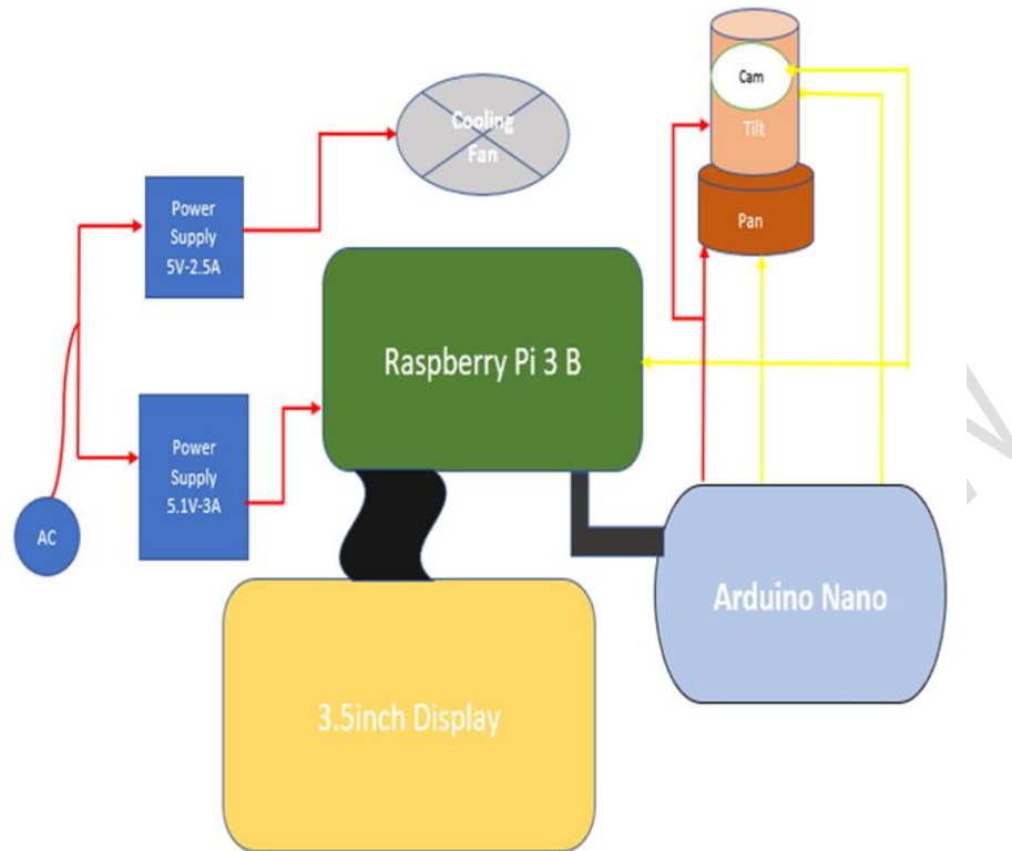
Fig. 11. Block diagram of hardware implementation.
