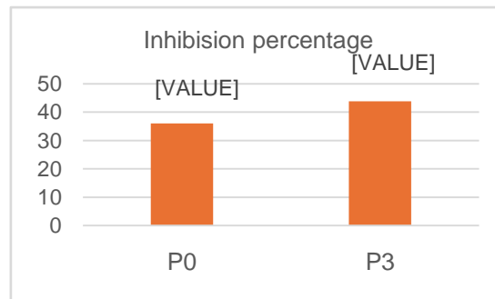
Figure 1. Percentage Inhibition of Samples Against DPPH
