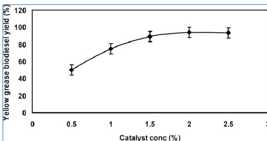
Fig 8: Biodiesel yield
