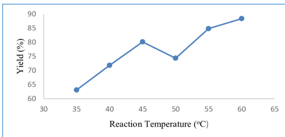
Fig 5: Variation of yield due to temperature fluctuations
