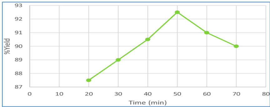
Fig 6 :Variation of yield due to reaction time
