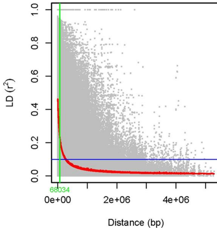
Figure 2. LD decay measured in association panel of 126 mungbean genotypes.
