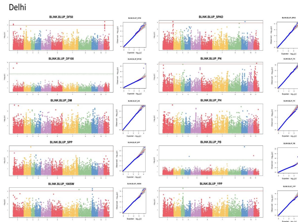
Figure 3. Manhattan (left) and quantile–quantile (Q–Q) (right) plots of various agronomic traits for (a) Delhi (b) Ludhiana.
