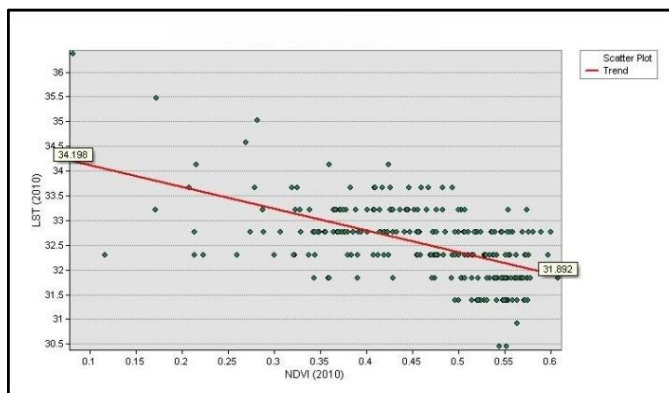
Figure 9. Correlation between LST and NDVI, 2010
