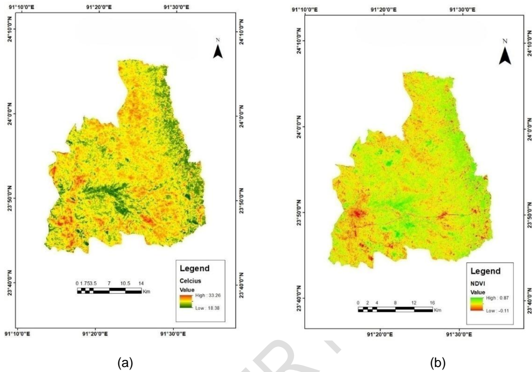
Figure 8. LST and NDVI map of West Tripura (a) LST, 2000 and (b) NDVI, 2000
