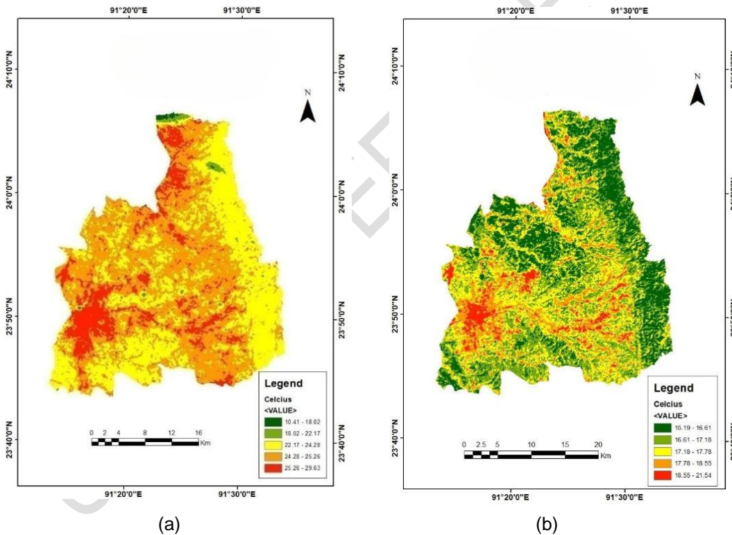
Fig.6. Land surface temperature of West Tripura(a) 2020, summer and (b) 2020, winter
