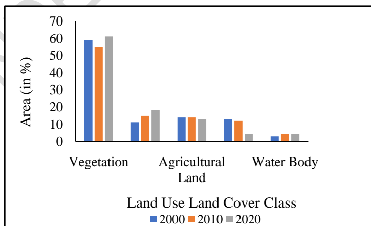
Fig. 2. Decadal wise percentage change in area of Land use land cover
