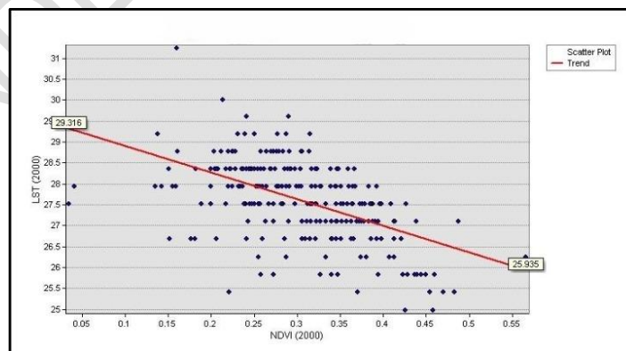
Figure 7. Correlation between LST and NDVI, 2000
