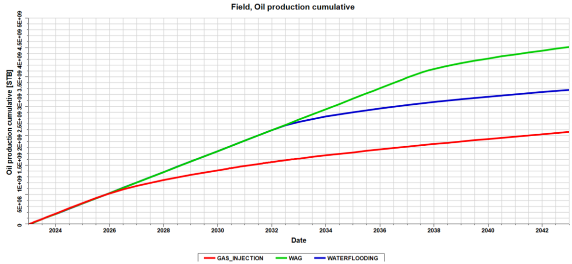
Fig.18: Plot of FOPT vs TIME (yrs) – Waterflooding, Gas and WAG Injection Table.12: FOPT Results for Waterflooding, Gas and WAG Injection
