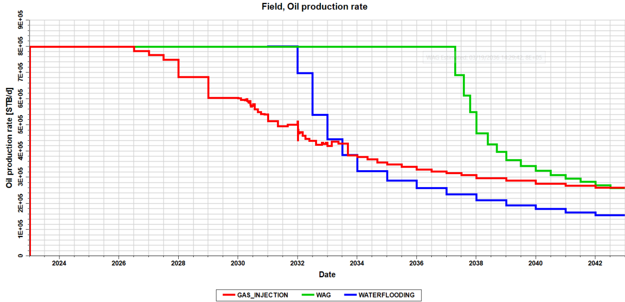
Fig. 17: Plot of FOPR vs TIME (yrs) – Waterflooding, Gas and WAG Injection
