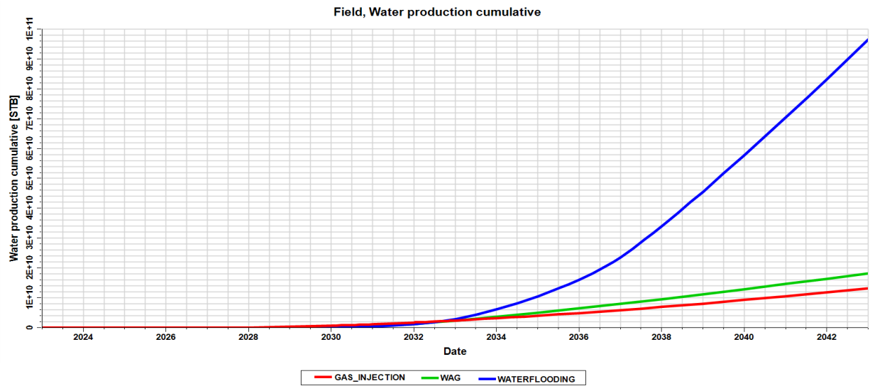
Fig.19: Plot of FWPT vs TIME (yrs) – Waterflooding, Gas and WAG Injections Table.13: FWPT Results for Waterflooding, Gas and WAG Injection
