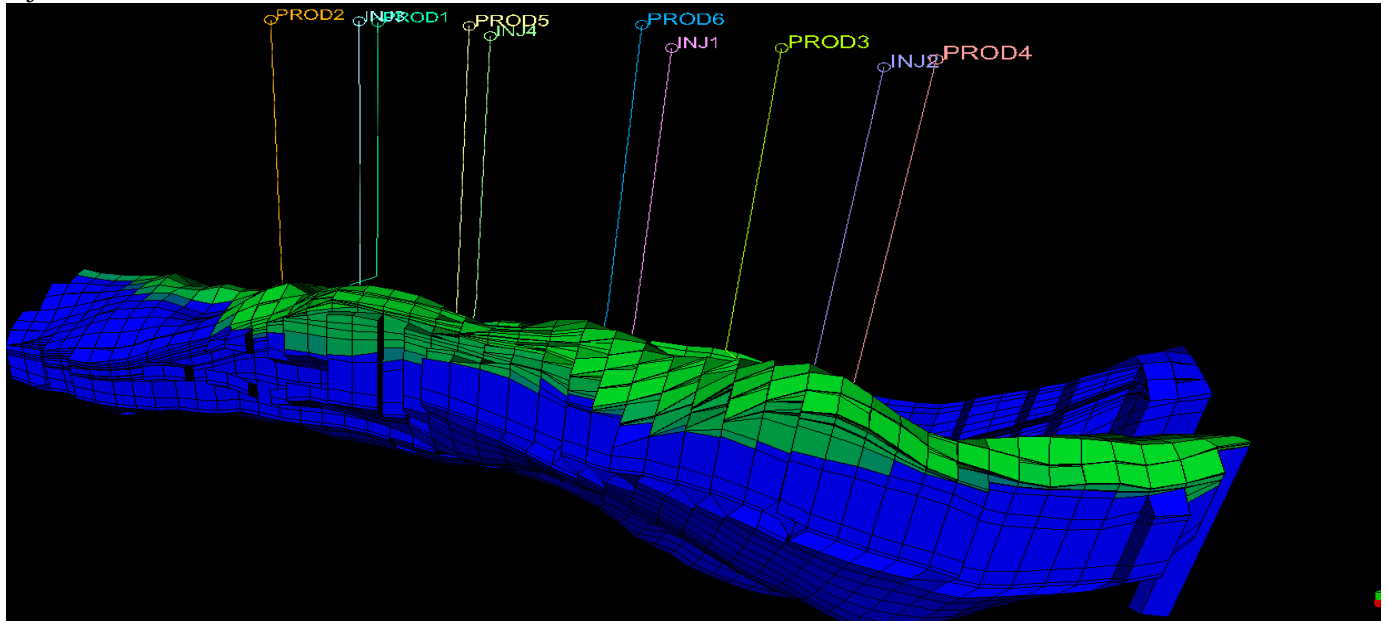
Fig.6: A 3D Model of Gas Injection
