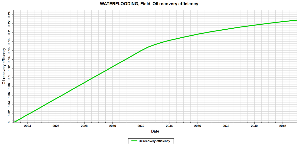
Fig. 10: Plot of FOE (Recovery Factor) vs TIME (yrs) – Water Injection WATERFLOODING, Field
