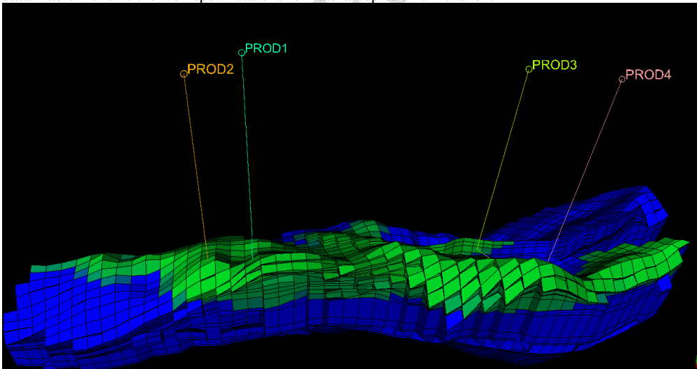
Fig.4:A3DModelofNaturalDepletion
