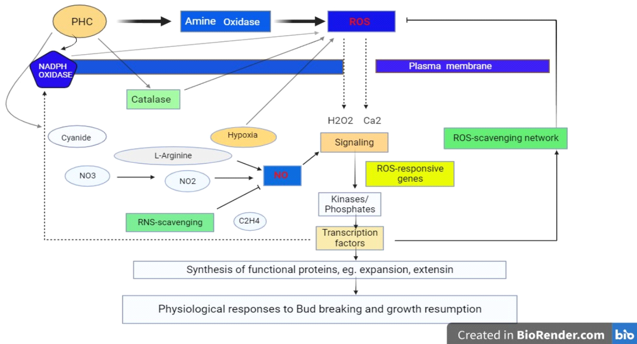
Fig 3: Physiological response to bud breaking and growth resumption.
