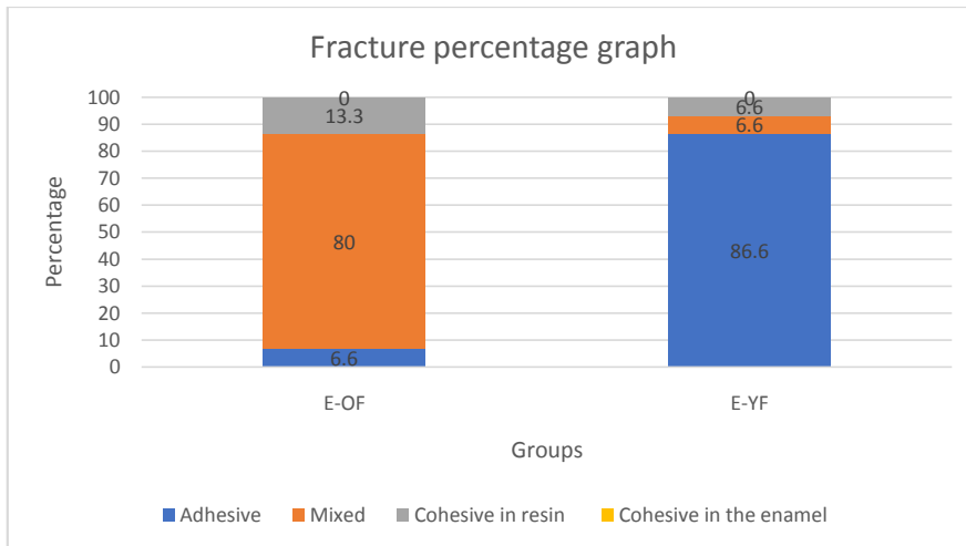
Graph 1. Percentage of fracture modes in the groups
