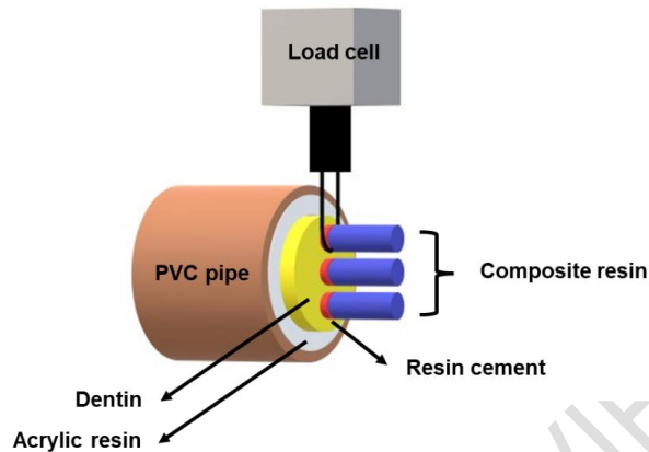
Figure 2 - Schematic view of the shear strength test
