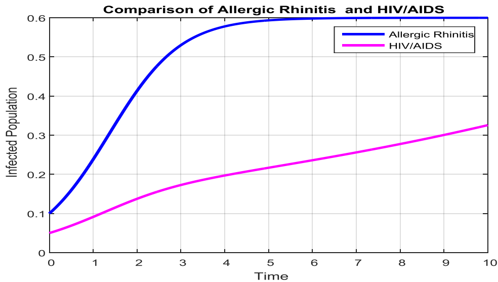
Figure 7: RK4 method
