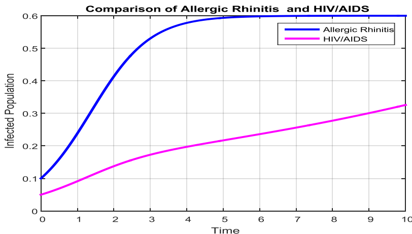
Figure 6: RK4 method
