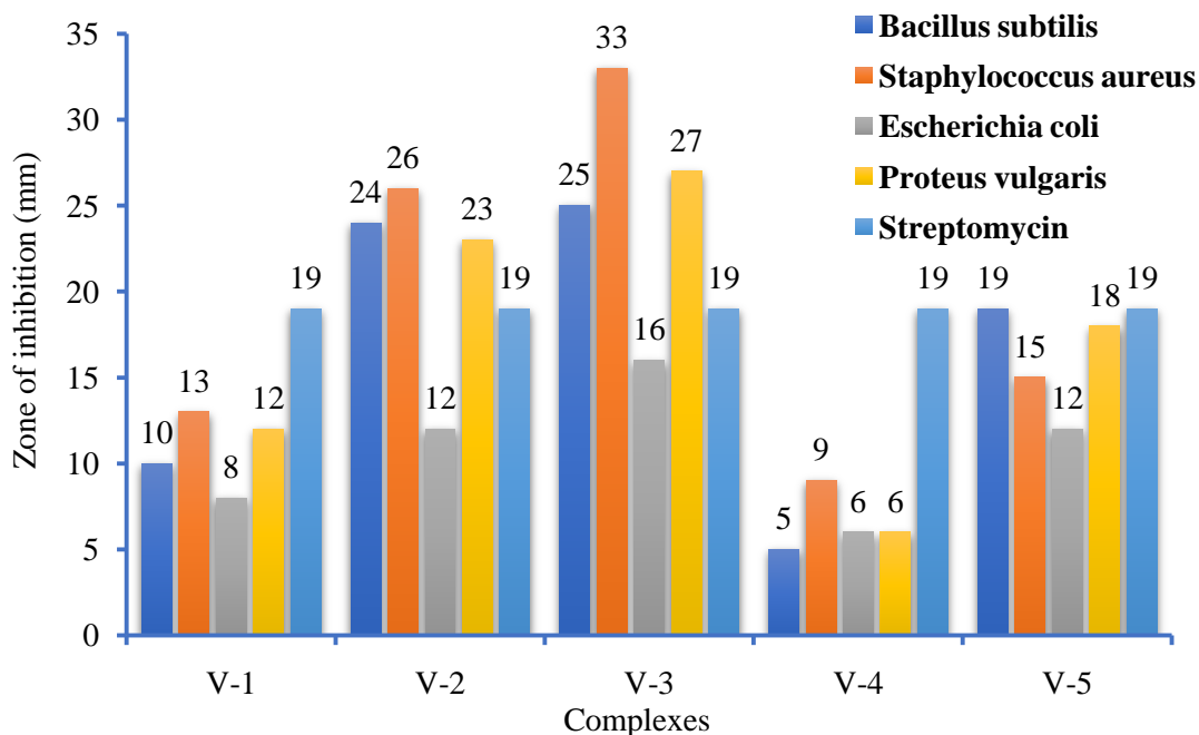
Figure 11: Graphical representation of antibacterial activity of oxovanadium(IV) complexes
