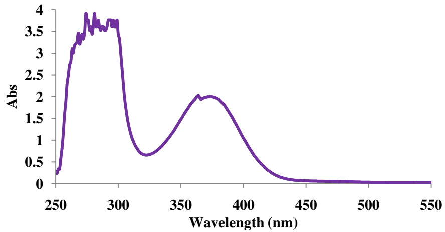
Figure 8: UV-Visible spectrum of [VO(sal-leu)(bpy)] complex, V-3
