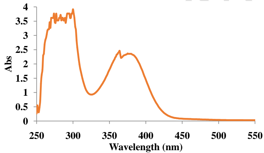
Figure 9: UV-Visible spectrum of [VO(sal-gly)(bpy)] complex, V-4
