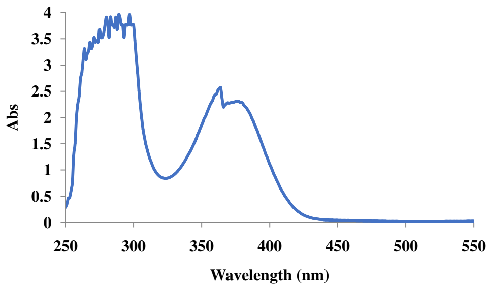
Figure 6 UV-Visible spectrum of [\text{VO}(\text{sal-ala})(\text{bpy})] complex, V-1
