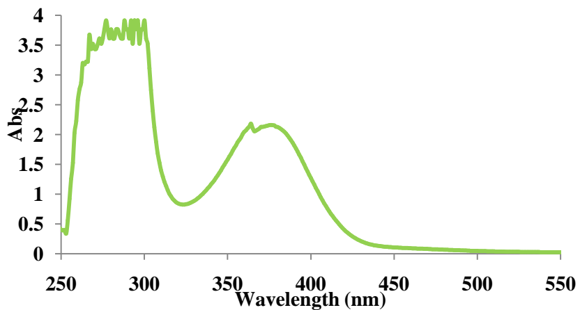
Figure 7 UV-Visible spectrum of [\text{VO}(\text{sal-pheala})(\text{bpy})] complex, V-2
