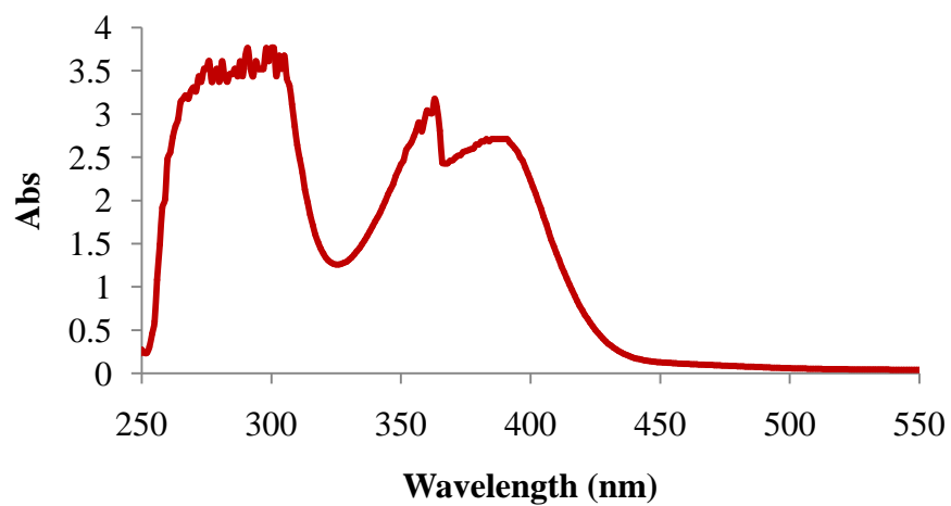
Figure 10: UV-Visible spectrum of [VO(sal-met)(bpy)] complex, V-5
