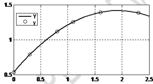
Figure 3. Approximation with the polyfit function
