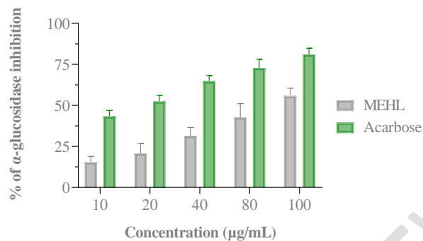
Figure 6: \alpha -glucosidase inhibition activity of MEHL. Results are expressed as mean \pm SD of three parallel measurements.
