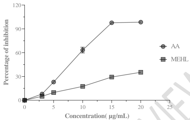
Figure 4: Scavenging activity of MEHL and ascorbic acid against ABTS radical. Results are expressed as
