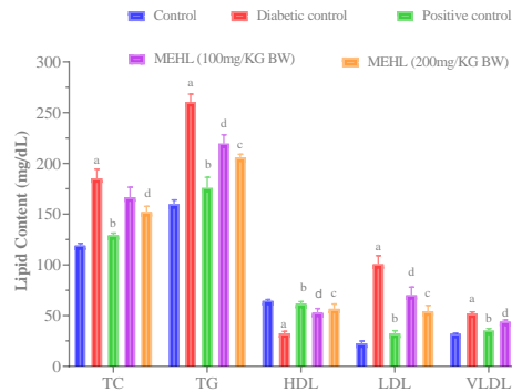
Figure 8: Effects of Methanol extract of H. schullileaf (MEHL) on lipid profile of diabetic mice after 21 days of treatment.
