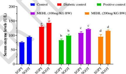
Figure 9: Effect of H. schulli leaf (MEHL) on serum SGPT and SGOT in diabetic mice after 21 days of treatment.
