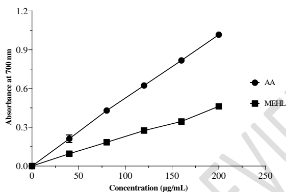
Figure 2: Ferric-reducing antioxidant activity of MEHL and ascorbic acid. Results are expressed as \text{mean} \pm \text{SD} of three parallel measurements.
