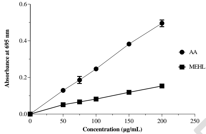
Figure 1: Total antioxidant capacity of MEHL and ascorbic acid (AA). Results are expressed as mean±SD of three parallel measurements.
