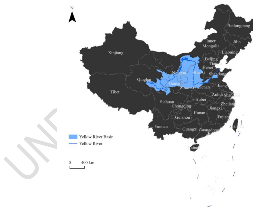
Figure 1. Location of Yellow River Basin
