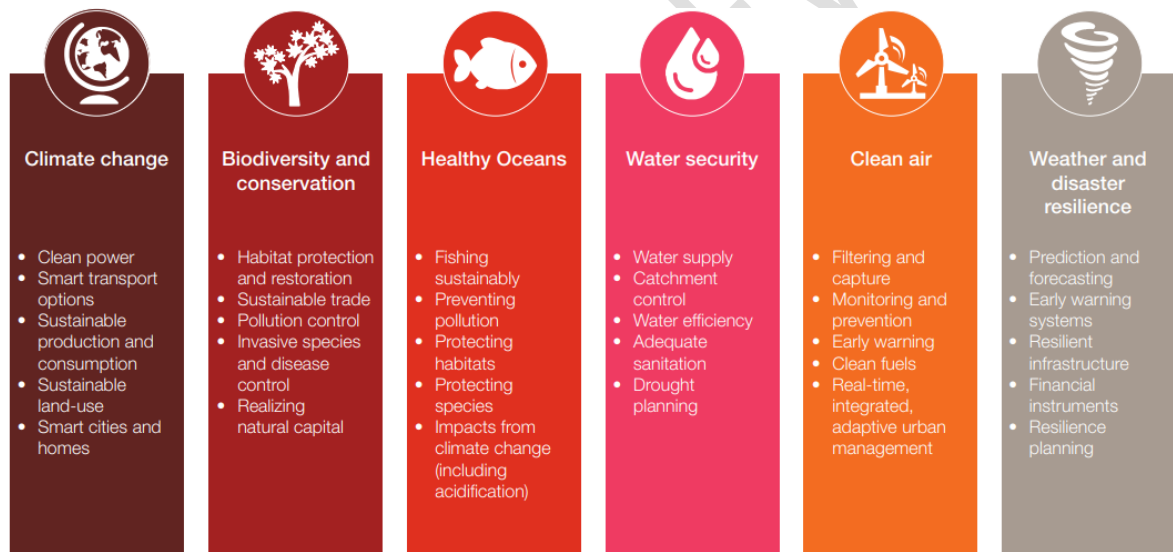
Figure 3. Priority action areas for addressing Earth challenge areas[23]
