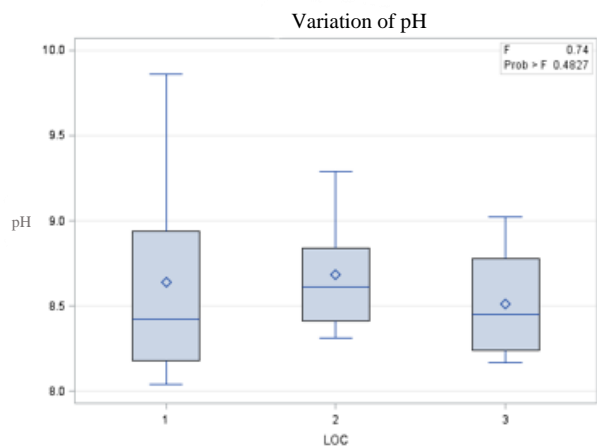
1.1 pH
