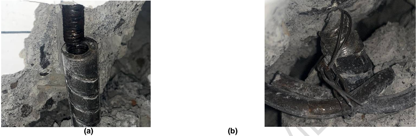
Fig. 14. (a) Failure at steel rebar thread (b) Steel rebar detached from coupler
