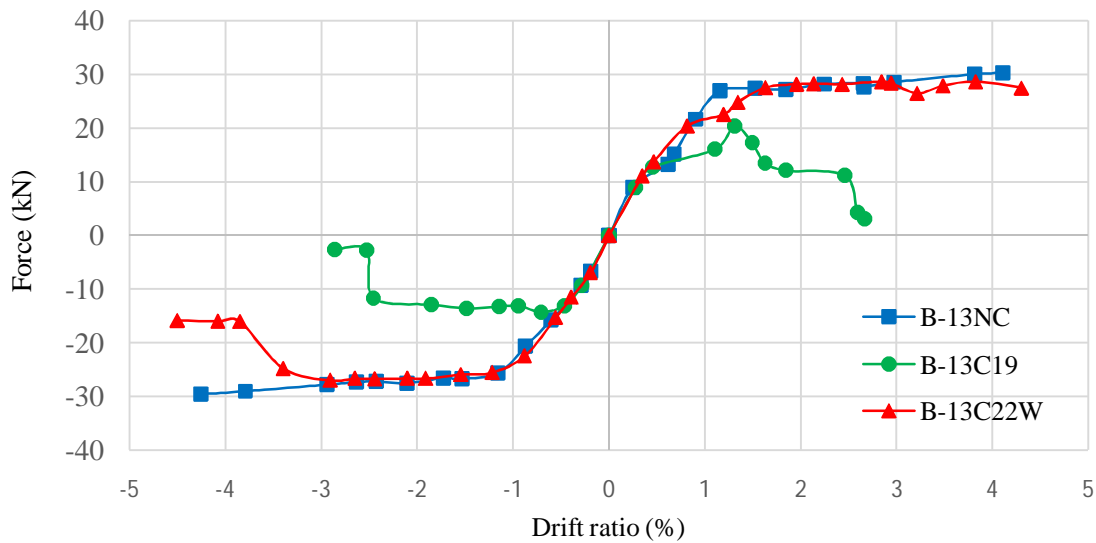
Fig. 7. Backbone curve
