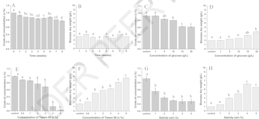
Fig. 3. Effects of (A and B) incubation time, (C and D) glucose concentration, (E and F) Tween 80 concentration, and (G and H) salinity on crude oil degradation by MG-07 and MG-07 biomass. Different lowercase letters above the bars indicate statistically different results.
