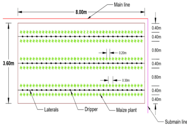
Fig. 1 Layout of each plot in the experiment
