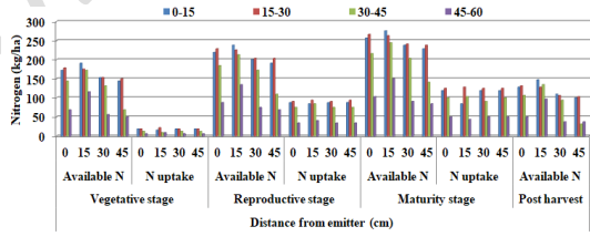
Fig. 24 Available N and N uptake in soil at different depths for I_3N_3 during rabi 2018-19
