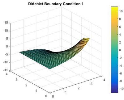
Exact
