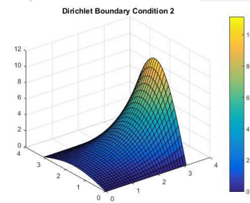
Approximate
