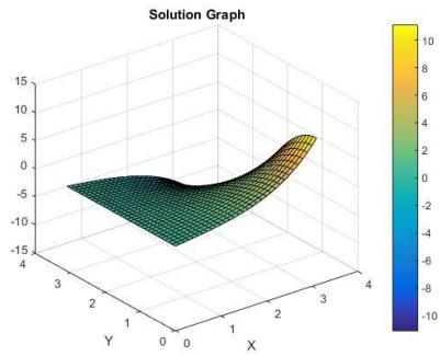
Approximate solution
