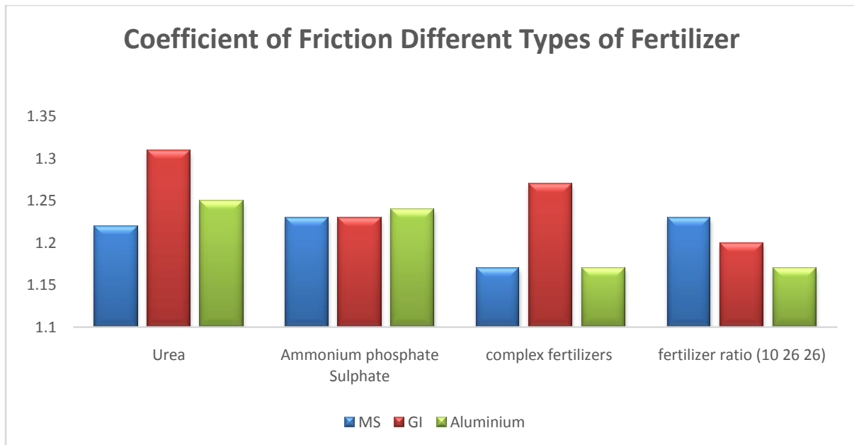
Fig.5 Coefficient of friction for granular fertilizers
