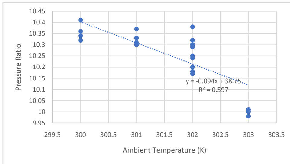
Fig. 2 Variation of ambient temperature on pressure ratio
