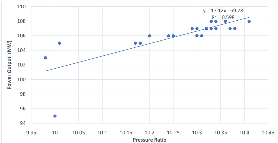
Fig. 4 Variation of pressure ratio on power output
