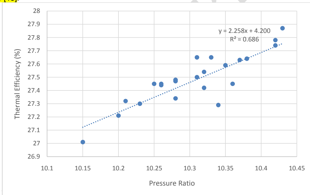
Fig. 3 Variation of pressure ratio on thermal efficiency
