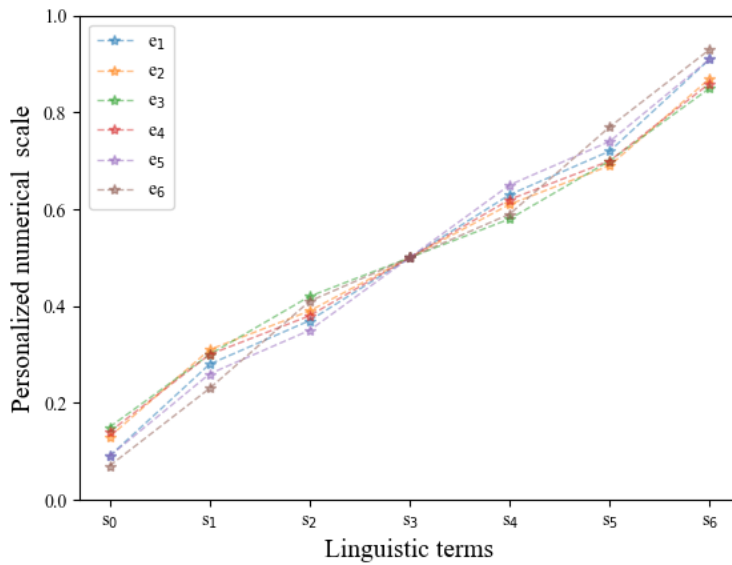
Figure 2: Numerical scales at round t = 0
