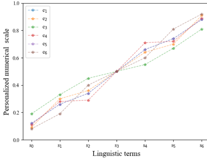
Figure 3: Numerical scales at round t = 1
