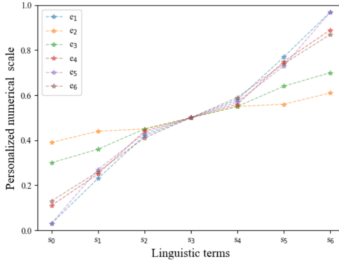
Figure 5: Numerical scales at round t = 3
