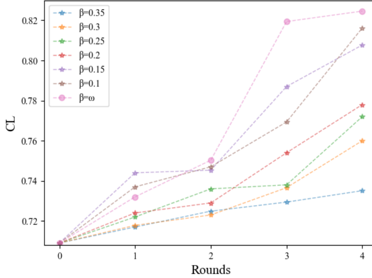
Figure 7: The result of comparison analysis on parameter \beta
