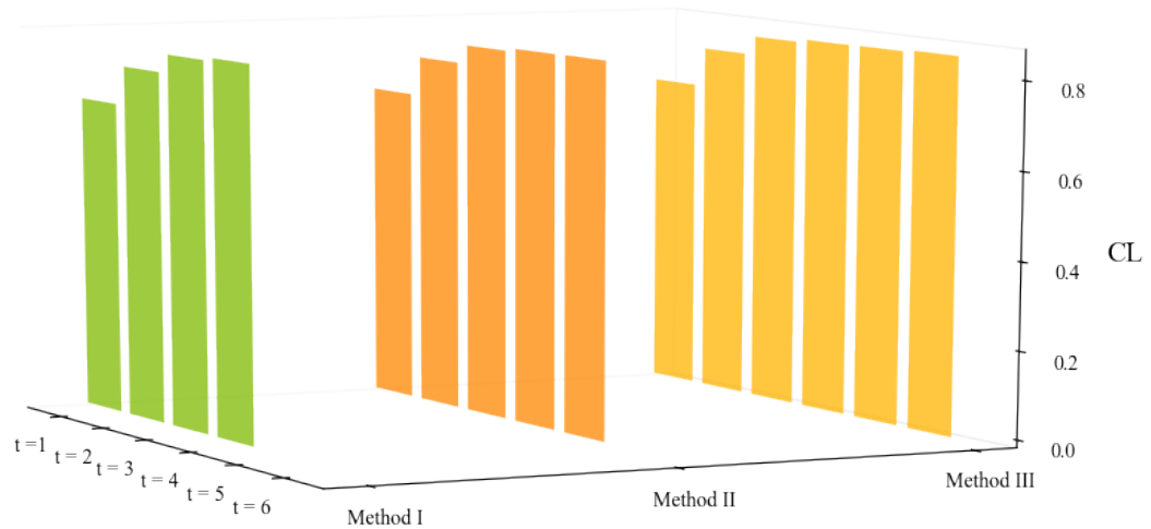
Figure 9: The result of comparison analysis on termination condition
