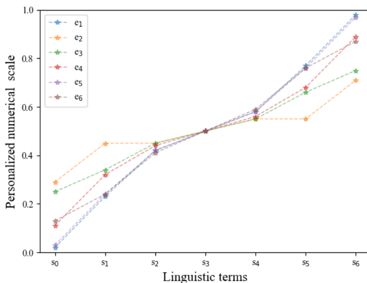
Figure 6: Numerical scales at round t = 4
