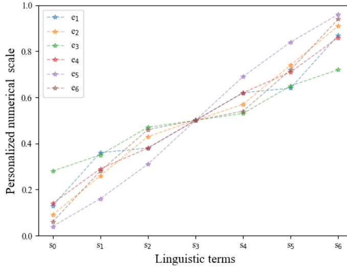
Figure 4: Numerical scales at round t = 2
