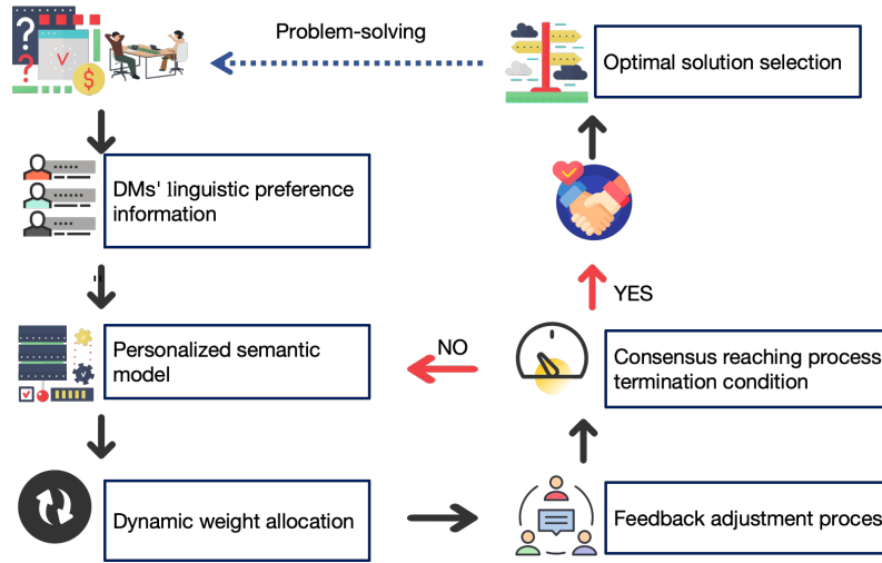
Figure 1: The Flowchart of Group Decision Method Based on Personalized Individualized Semantic Continuous Learning
