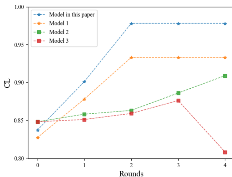
Figure 8: Comparison of continuous learning with adaptive weight allocation
